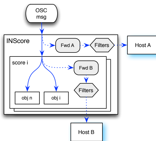
Figure 3. Message forwarding mechanism.
